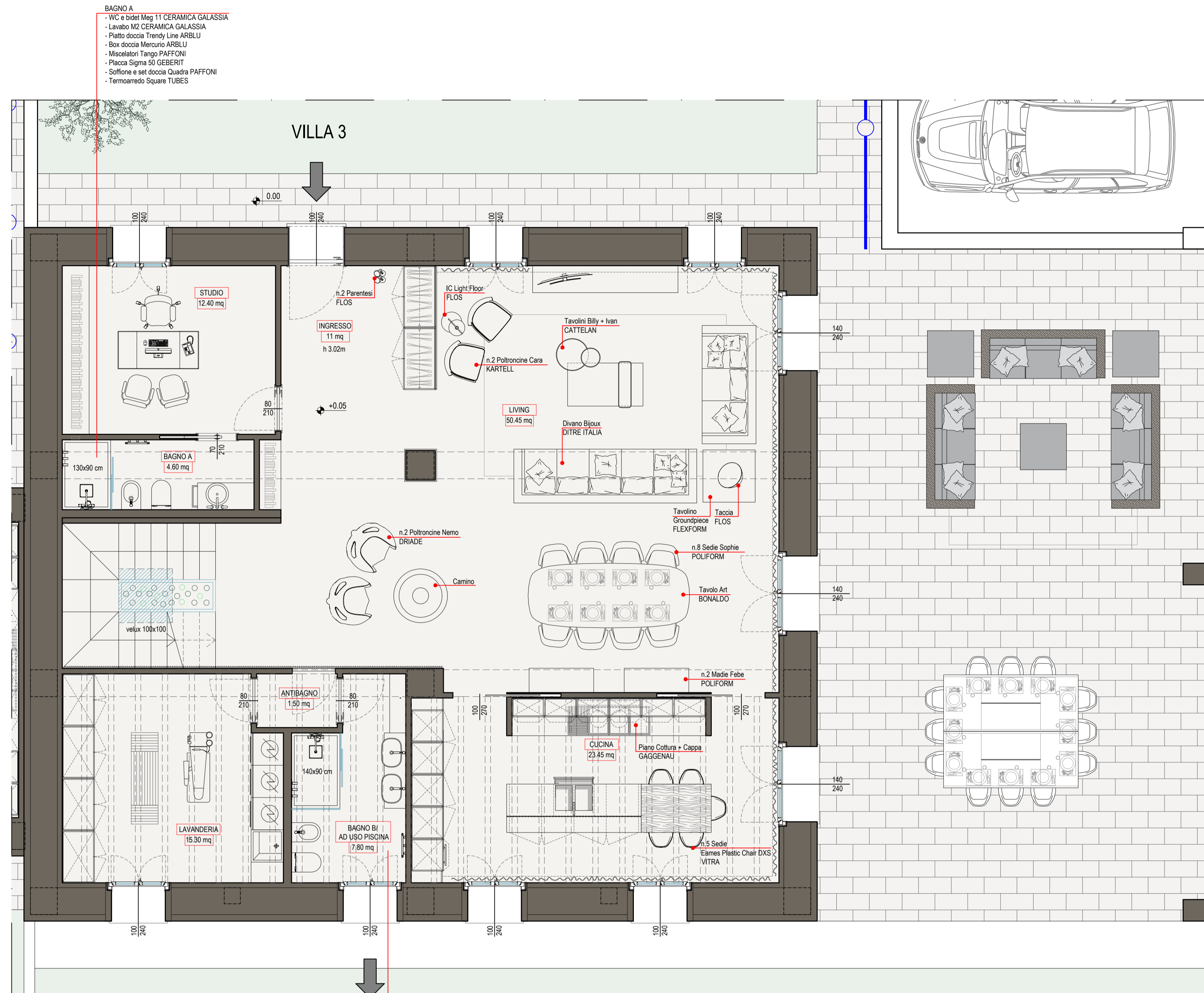
VILLA 3 - PIANO TERRA
