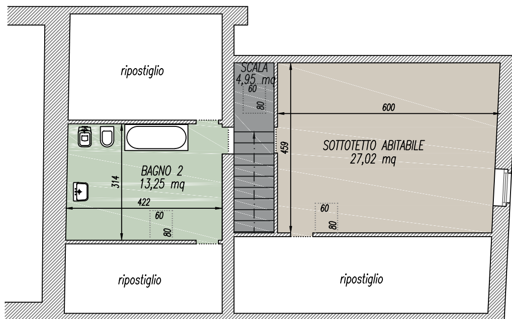
MANSARDA
