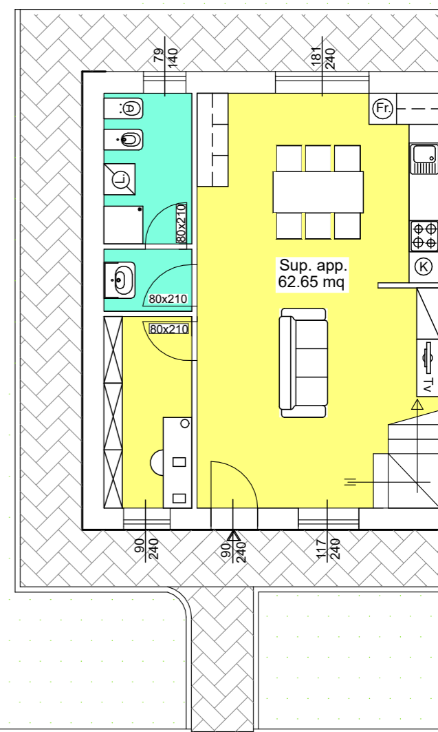
PIANO TERRA
