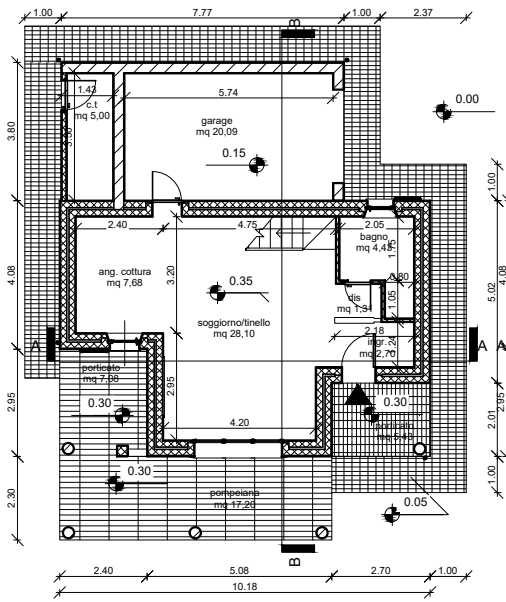
PIANO TERRA
