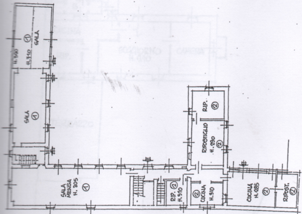
PIANO TERRA
