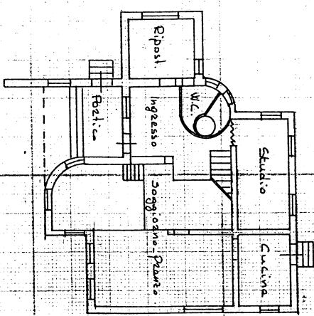
PIANO TERRA M=2.70
