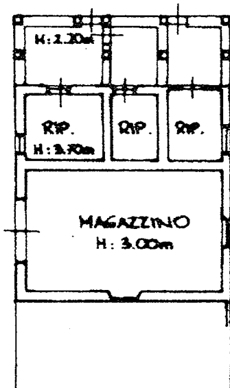
PIANO TERRA
