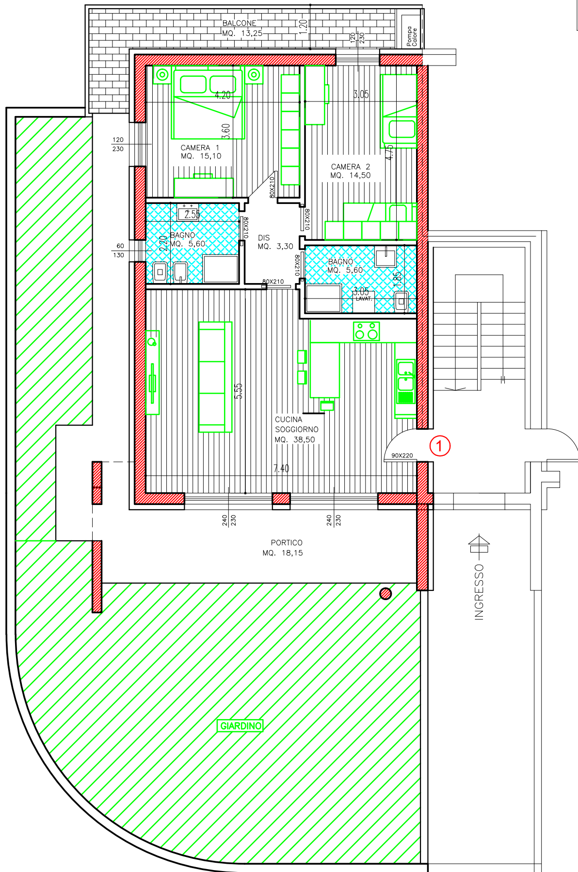
PIANO TERRA 1:100
