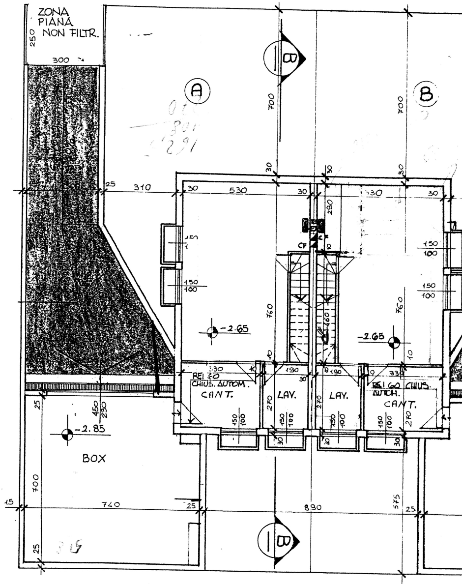
PIANO INTERRATO
