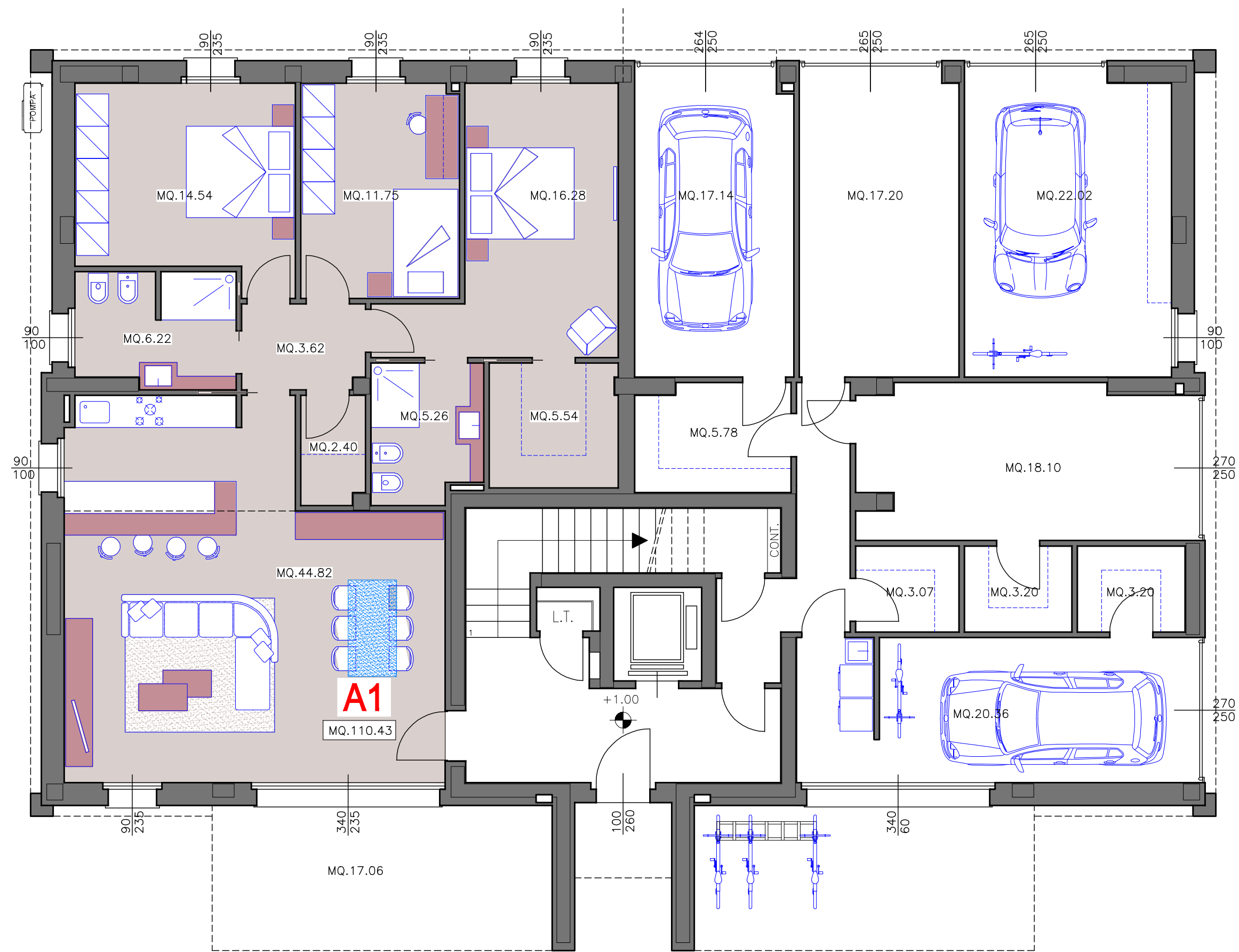
PIANO TERRA H=270
