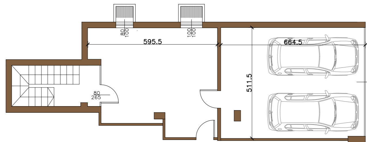
PIANO INTERRATO
