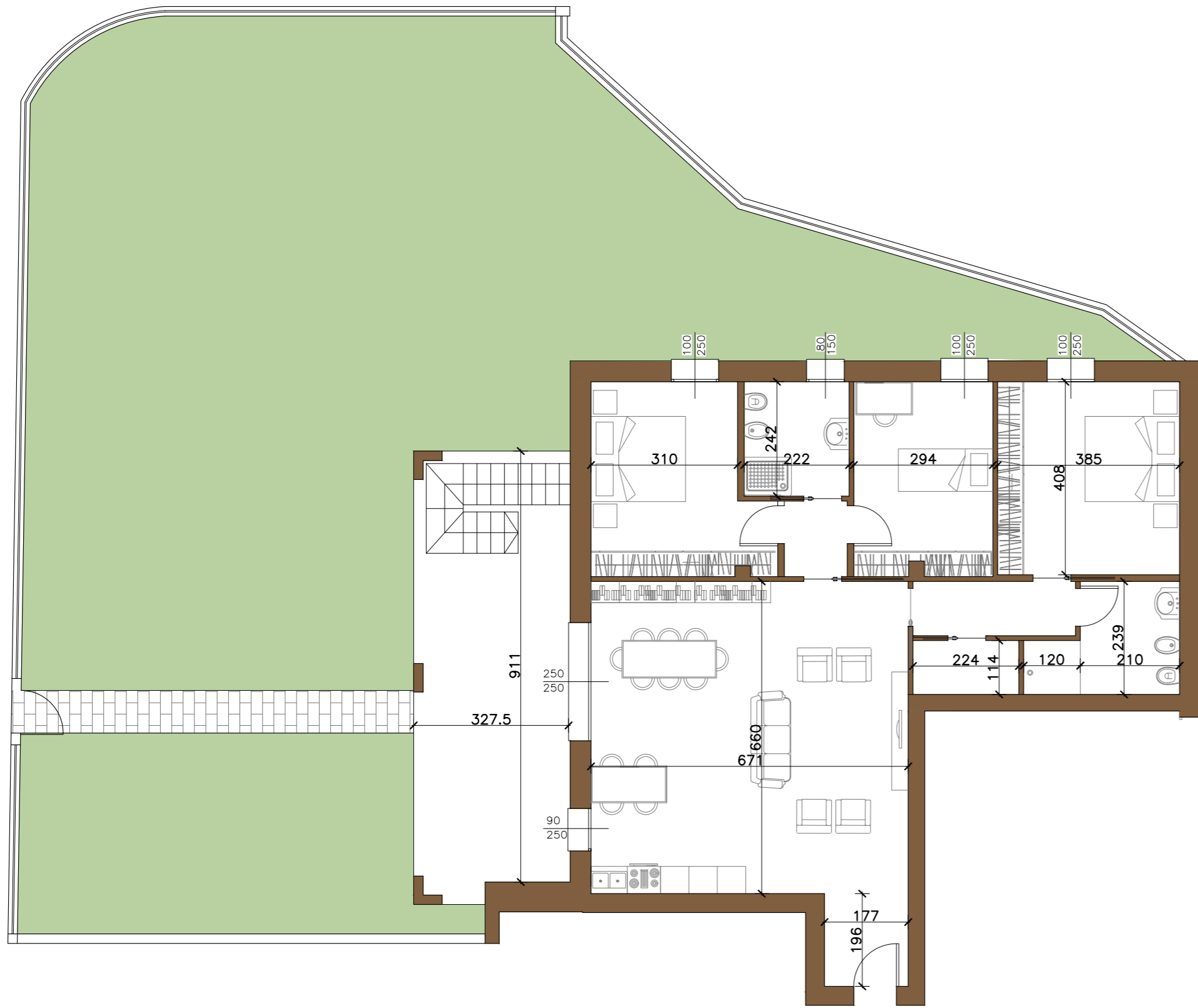
PIANO TERRA
