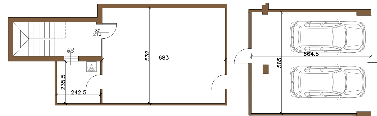
PIANO INTERRATO
