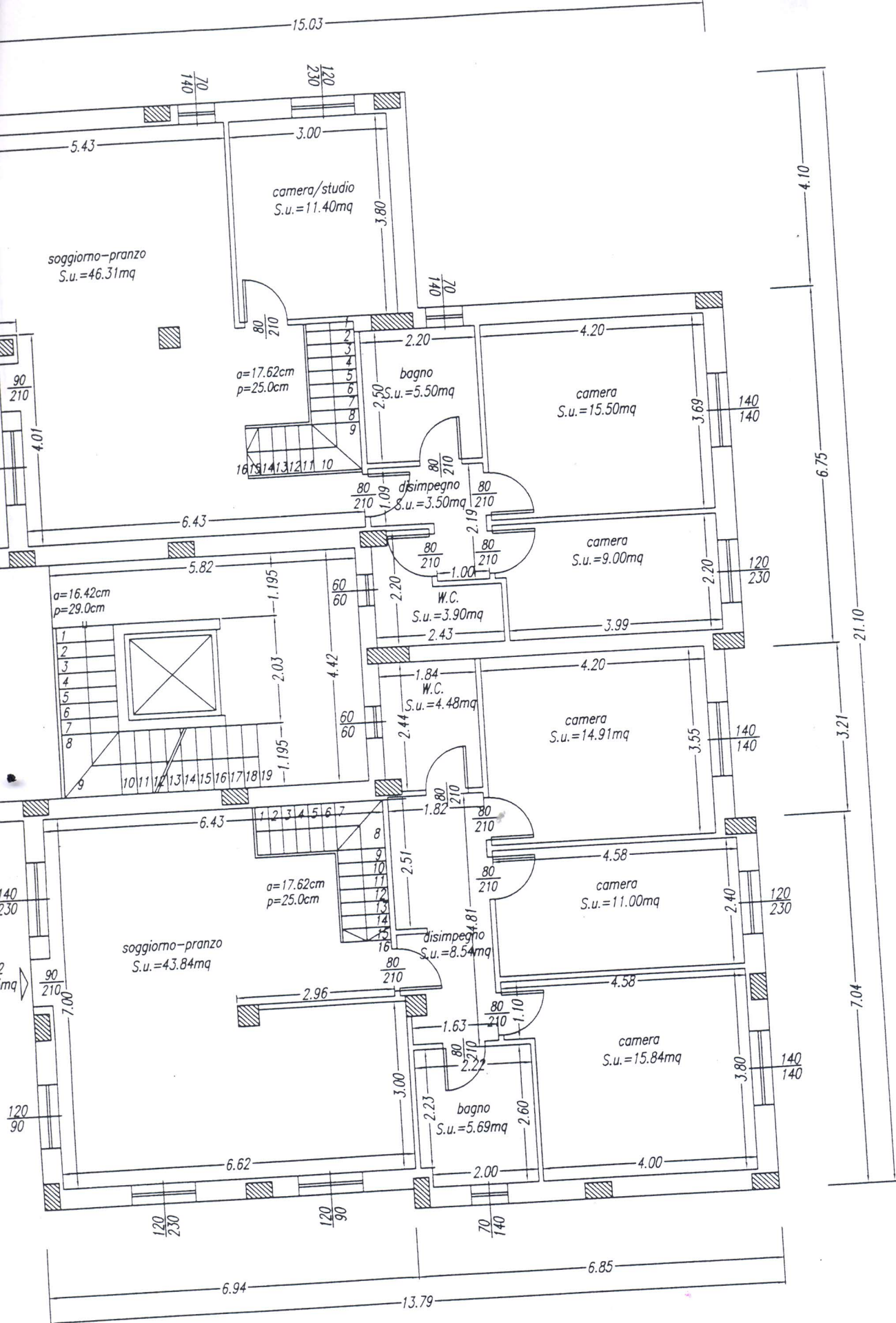
PIANTA PIANO TERRA (Q.+0.00) scala 1:100
