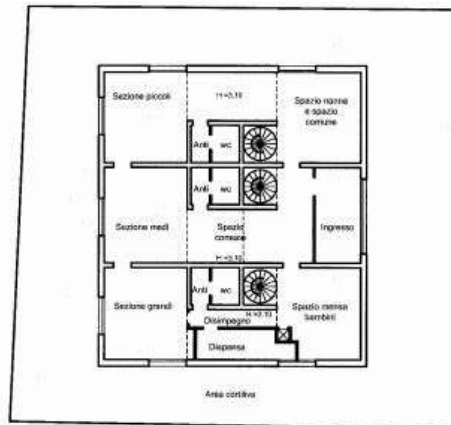
PIANO TERRA
