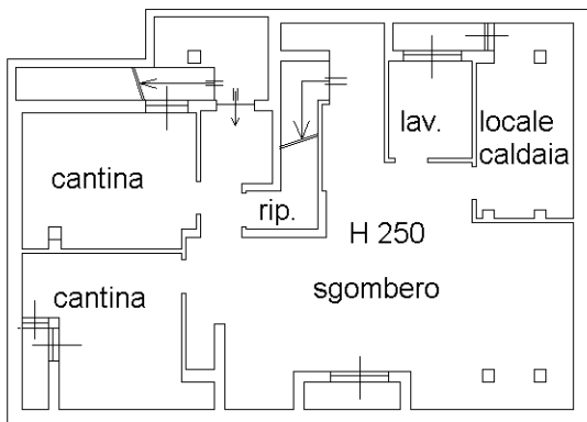
PIANO INTERRATO
