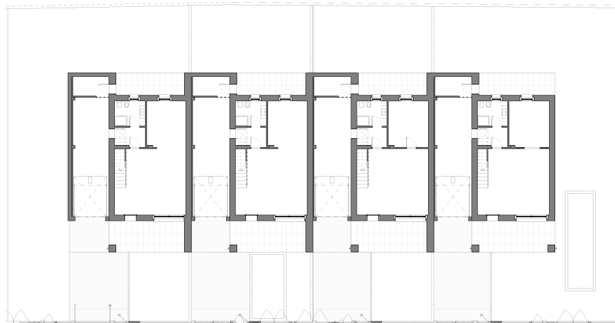
1 Planimetria piano terra
