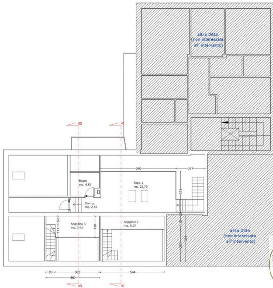
piano soppalco
