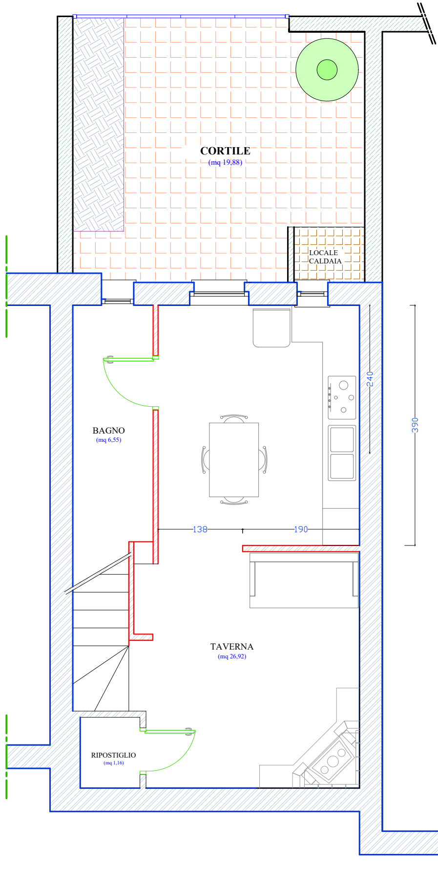
PIANO SEMINTERRATO (mq 34,63)
