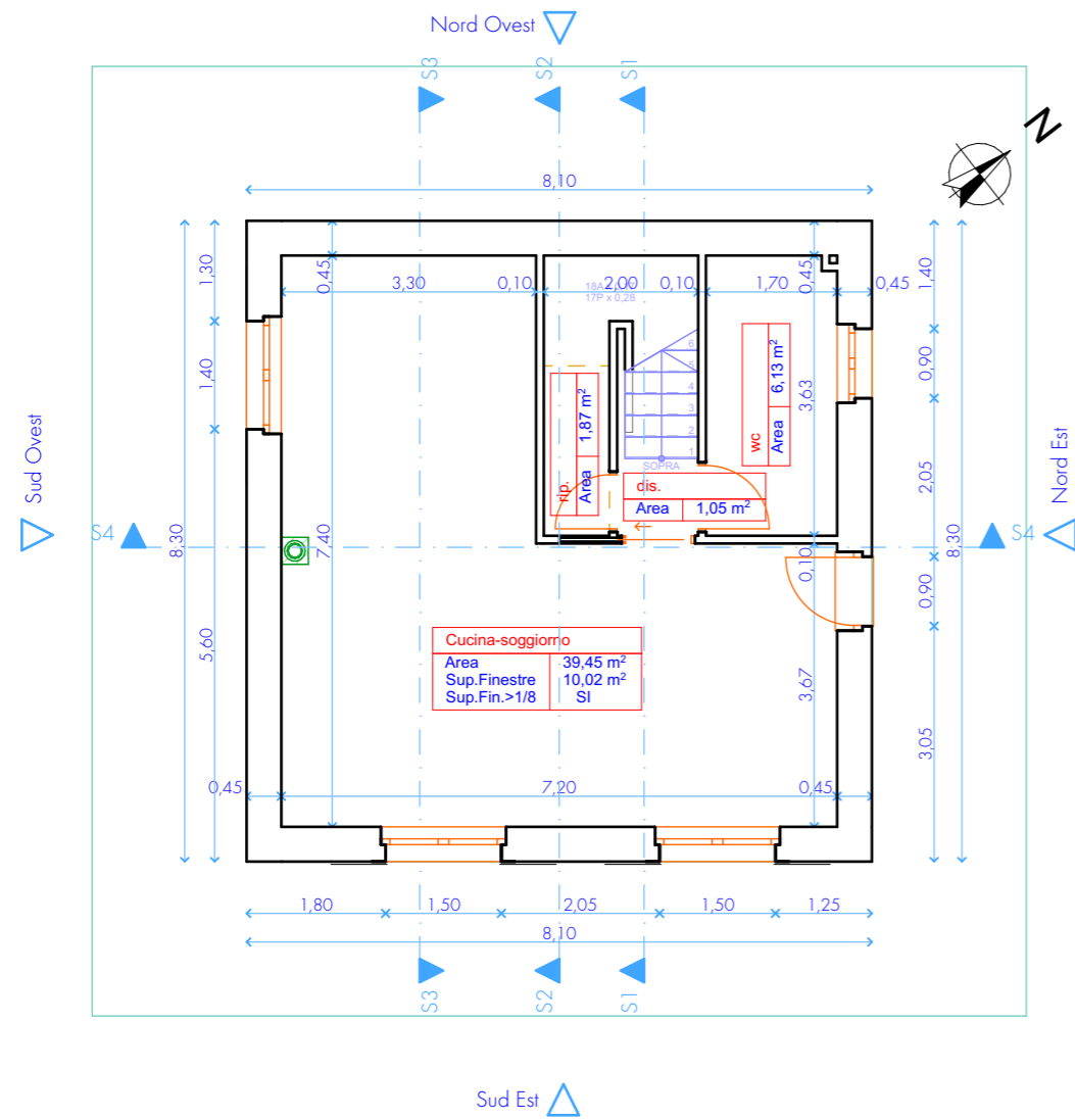
0. Piano Terra 1:100
