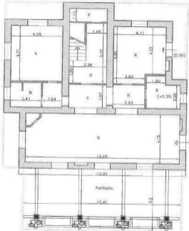
Piano Terra scala 1 : 100
