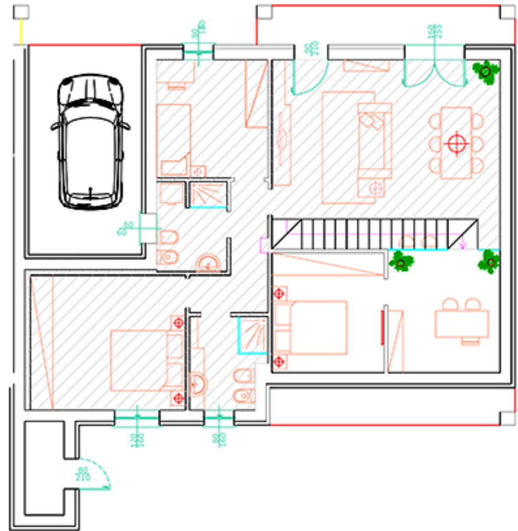
piano soppalco in pianta
