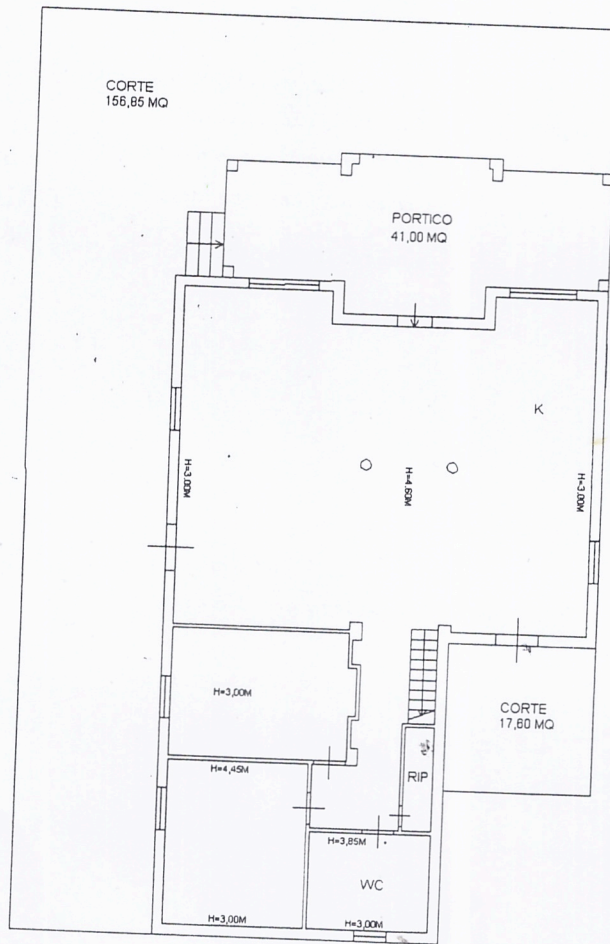
PIANO TERRA
