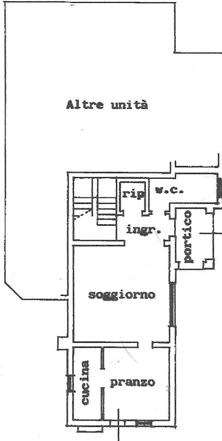
PIANTA PIANO TERRA H = 2.70
