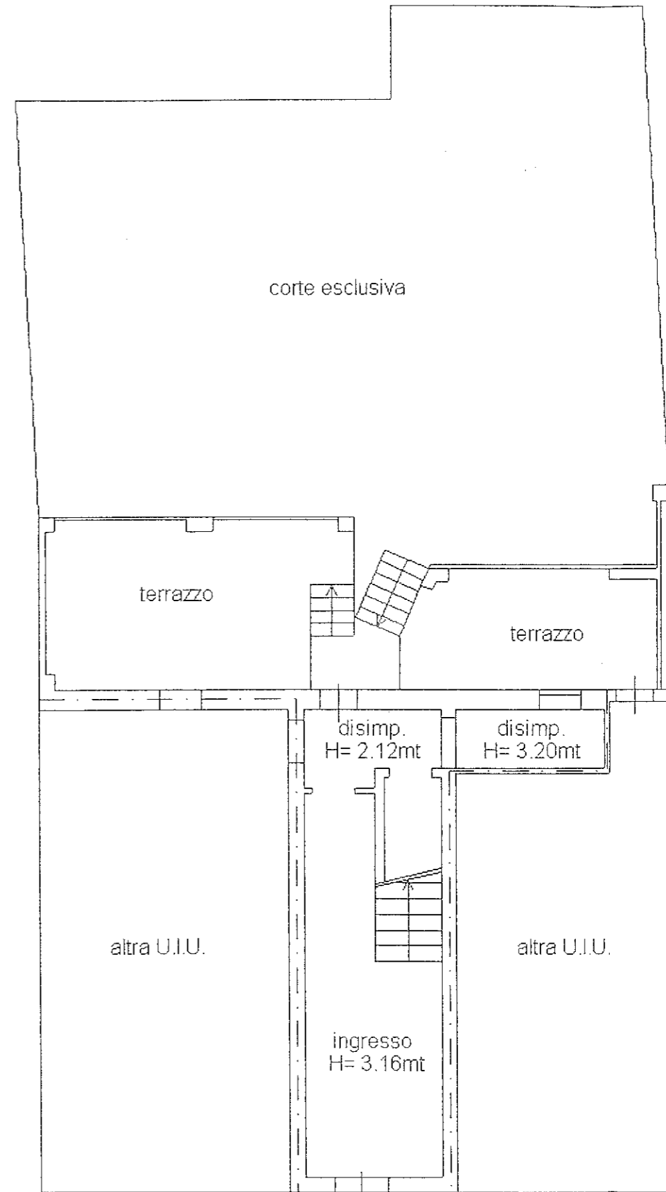
PIANO TERRA
