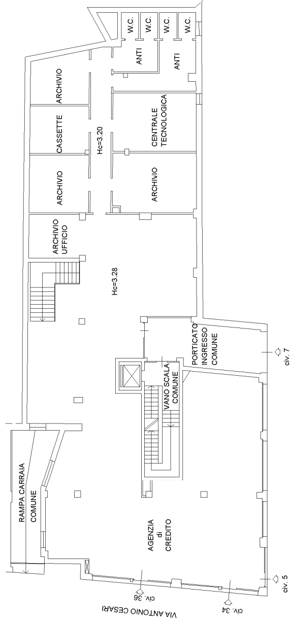
PIANO TERRA
