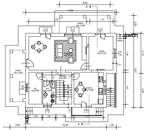
PIANO INTERRATO
