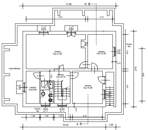
PIANO TERRA
